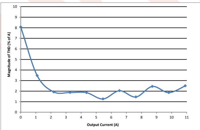
Figure 17: Total harmonic distortion (THD) at 115Vrms, 60Hz vs. output current (Tested with APFIC module and ACF-U-230-HT filter).
