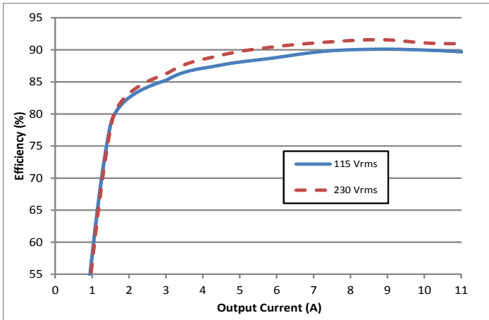
Figure 1: Efficiency at nominal output voltage vs. output current for 115Vrms and 230Vrms input voltage (applies to both 60Hz and 400Hz) at T_b = 25^\circ\text{C} .
