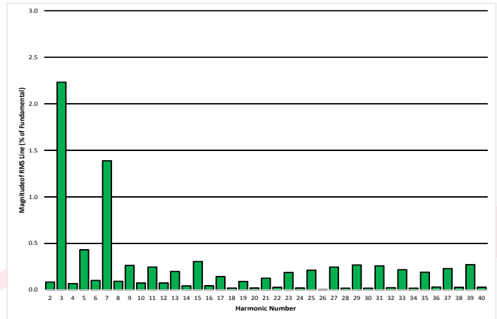
Figure 20: Input current harmonic components at full load, 115Vrms 400 Hz, T=25°C (Tested with APFIC module and ACF-U-230-HT filter).
