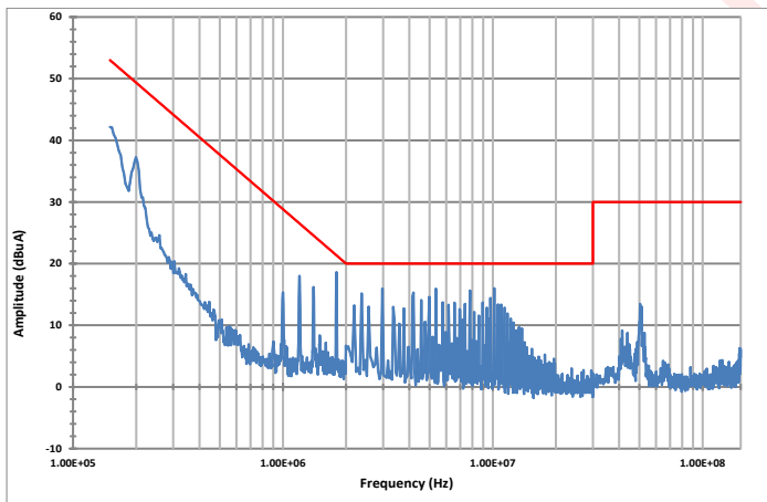
Figure 21: D0-160G conducted emissions of ACF-U-230-HT filter and APFIC-U converter at full load, 115Vrms 400 Hz, category M limit.
