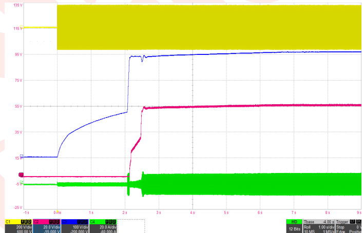
Figure 4: Typical startup waveform with 600µF hold-up capacitor (115Vrms, 400Hz) Ch1: V_{in} (200V/div), Ch2: V_{out} (20V/div), Ch3: Hold-up capacitor voltage (100V/div), Ch4: I_{in} (20A/div), Timebase: (1s/div).
