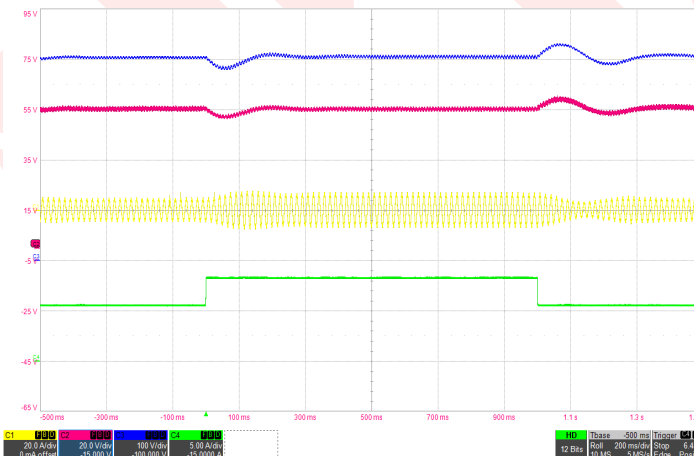
Figure 5: Load transient with 600µF hold-up capacitor (50%-75%-50% of I_{max} , 115Vrms, 60Hz) Ch1: I_{in} (20A/div), Ch2: V_{out} (20V/div), Ch3: Hold-up capacitor voltage (100V/div), Ch4: I_{out} (5A/div), Timebase: (200ms/div).
