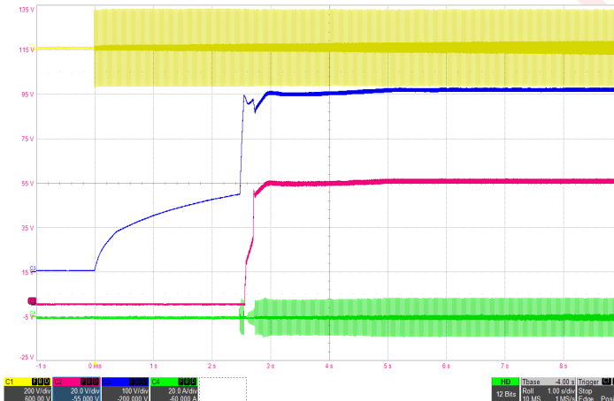
Figure 3: Typical startup waveform with 600µF hold-up capacitor (115Vrms, 60Hz) Ch1: V_{in} (200V/div), Ch2: V_{out} (20V/div), Ch3: Hold-up capacitor voltage (100V/div), Ch4: I_{in} (20A/div), Timebase: (1s/div).
