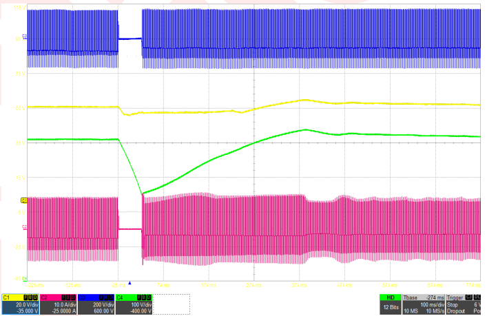
Figure 10: Line drop out with 600µF hold-up capacitor at full load (115Vrms, 400Hz) Ch1: Vout (20V/div), Ch2: Iin (10A/div), Ch3: Vin (200V/div), Ch4: Vhold-up (100V/div), Timebase: (100ms/div).
