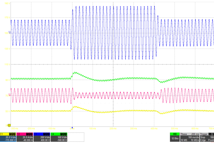
Figure 7: Input transient with 600µF hold-up capacitor at full load (115Vrms-220Vrms-115Vrms, 60Hz) Ch1: Vout (20V/div), Ch2: Iin (20A/div), Ch3: Vin (200V/div), Ch4: Vhold-up (100V/div), Timebase: (100ms/div).
