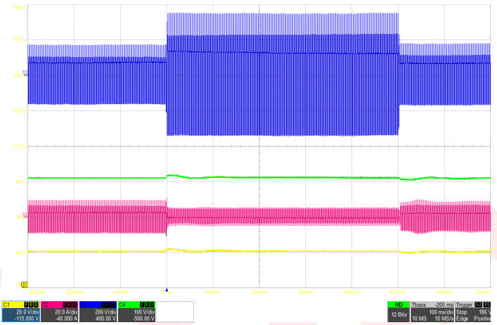
Figure 8: Input transient with 600µF hold-up capacitor at full load (115Vrms-220Vrms-115Vrms, 400Hz) Ch1: Vout (20V/div), Ch2: Iin (20A/div), Ch3: Vin (200V/div), Ch4: Vhold-up (100V/div), Timebase: (100ms/div).
