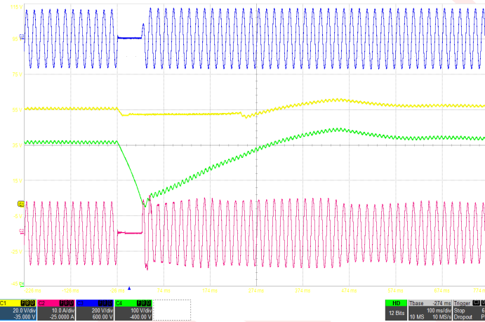
Figure 9: Line drop out with 600µF hold-up capacitor at full load (115Vrms, 60Hz) Ch1: Vout (20V/div), Ch2: Iin (10A/div), Ch3: Vin (200V/div), Ch4: Vhold-up (100V/div), Timebase: (100ms/div).
