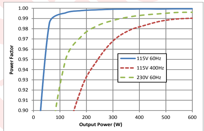
Figure 22: Power factor vs. output power at different input conditions, T=25°C (Tested with APFIC module and ACF-U-230-HT filter).
