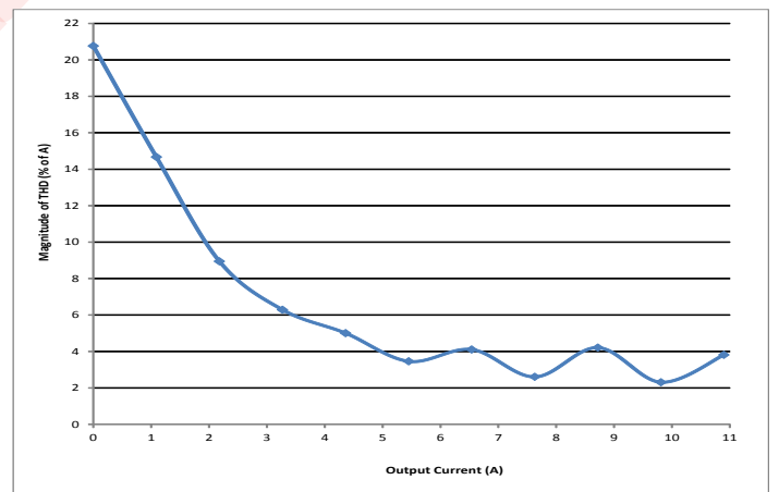
Figure 18: Total harmonic distortion (THD) at 115Vrms, 400Hz vs. output current (Tested with APFIC module and ACF-U-230-HT filter).
