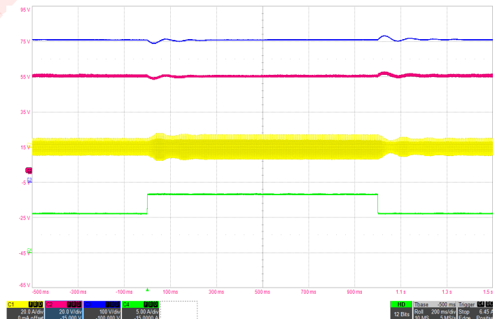
Figure 6: Load transient with 600µF hold-up capacitor (50%-75%-50% of I_{max} , 115Vrms, 400Hz) Ch1: I_{in} (20A/div), Ch2: V_{out} (20V/div), Ch3: Hold-up capacitor voltage (100V/div), Ch4: I_{out} (5A/div), Timebase: (200ms/div).
