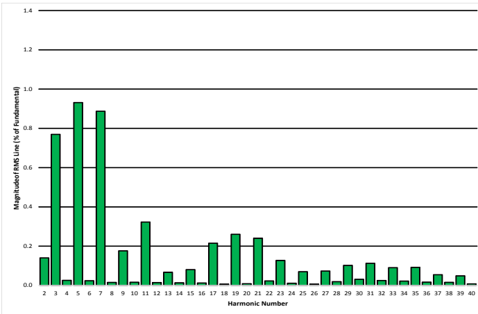
Figure 19: Input current harmonic components at full load, 115Vrms 60 Hz, T=25°C (Tested with APFIC module and ACF-U-230-HT filter).
